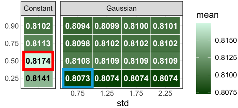
Sensitivity
