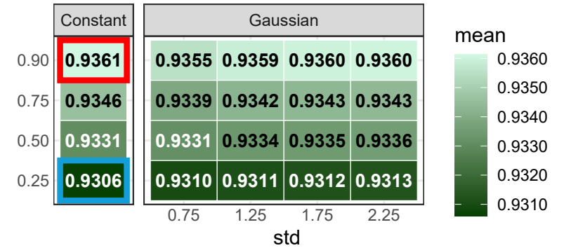
Specificity
