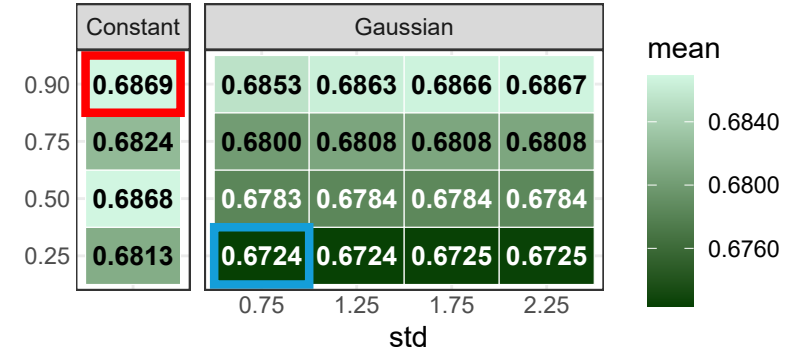
Specificity
