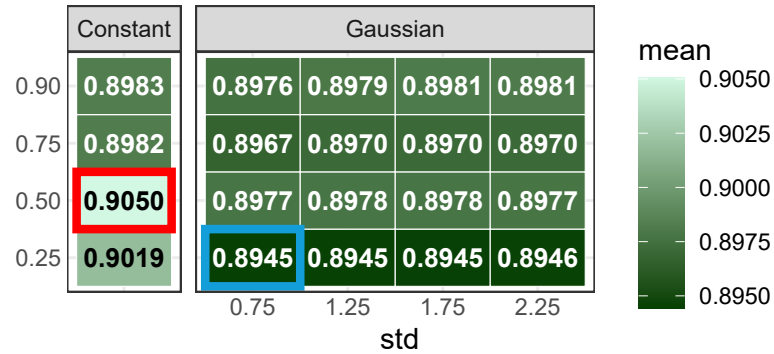
Sensitivity
