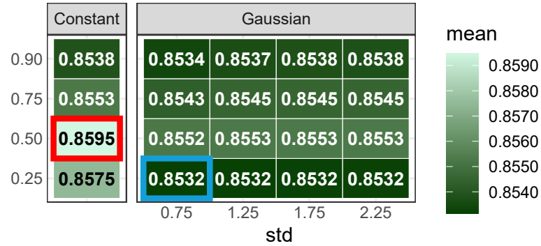
Jaccard
